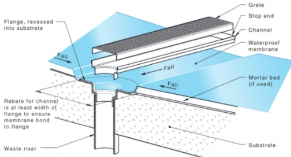
Figure 4.3.2 — Linear drain single outlet centrally located
