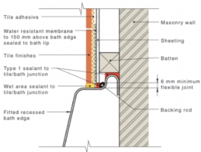
Figure 4.13.2.2(B) — Bath with no shower over it — Fitted bath — Masonry wall with sheet spaced via battens
