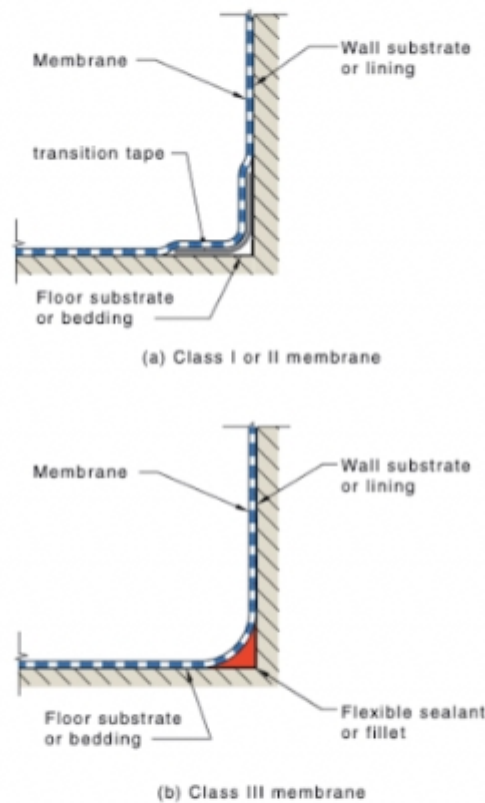
Figure 4.10 — Typical transition tape details
