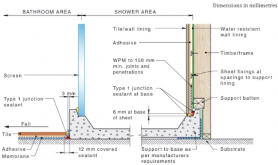
Figure 4.14(A) — Section through stud wall with self-supporting prefinished wall panels and preformed or cast shower bases
