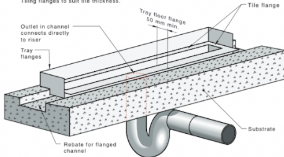
Figure A.6(D) — Fabricated flange components explanatory diagram
