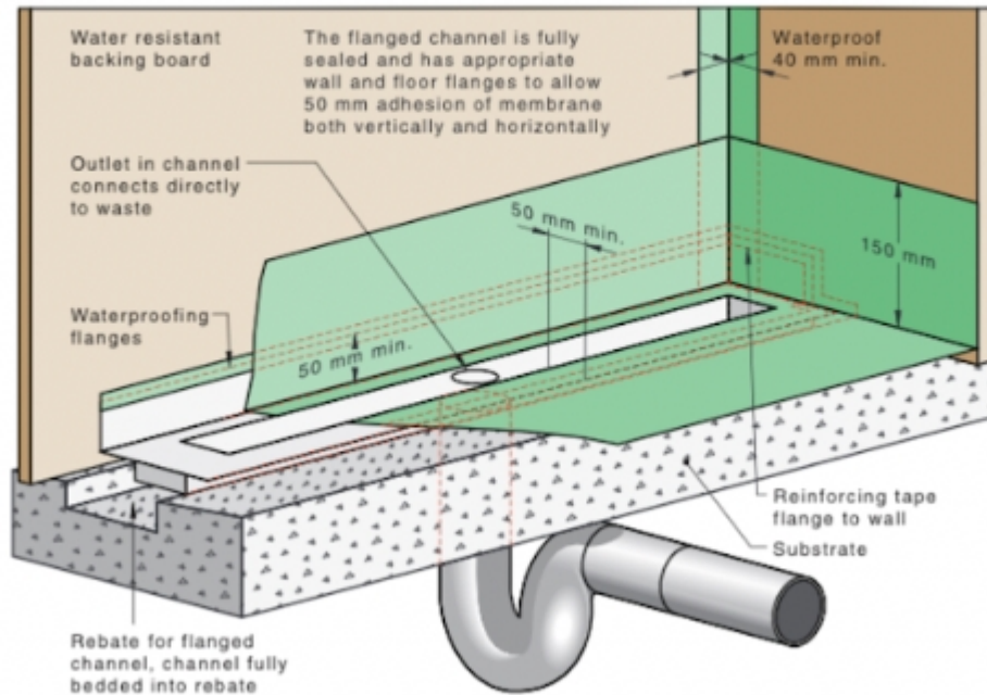
Figure A.6(C) — Custom fabricated flanged channel against a wall
