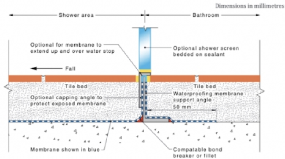
Figure 4.8.2(D) — Shower waterstop and cover angle
