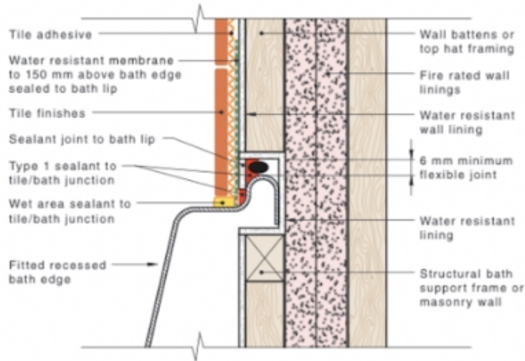
Figure 4.13.2.2(E) — Bath with no shower over it — Fitted bath — Fire rated framed wall
