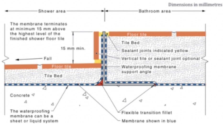
Figure 4.8.2(C) — Step-down shower waterstop and cover angle
