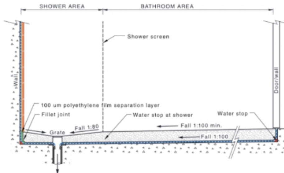
Figure 4.17 — Polished concrete floor for unenclosed shower
